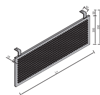
Perforirani hrbet mize 21
